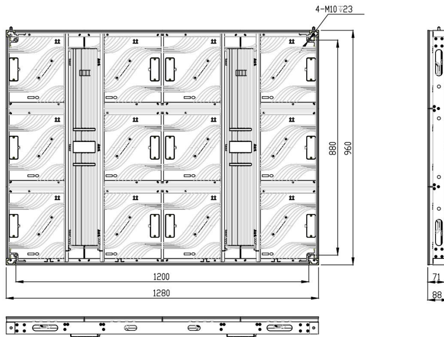
1 Standard cabinet: 1280 x 960mm
